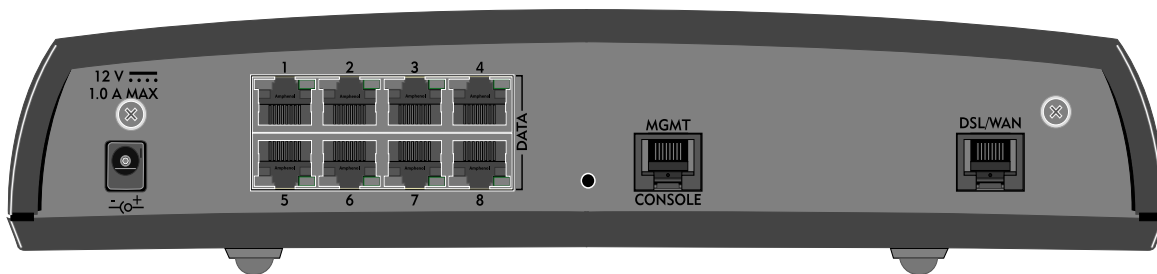
Figure 4-2: 5950 Router Back Panel
